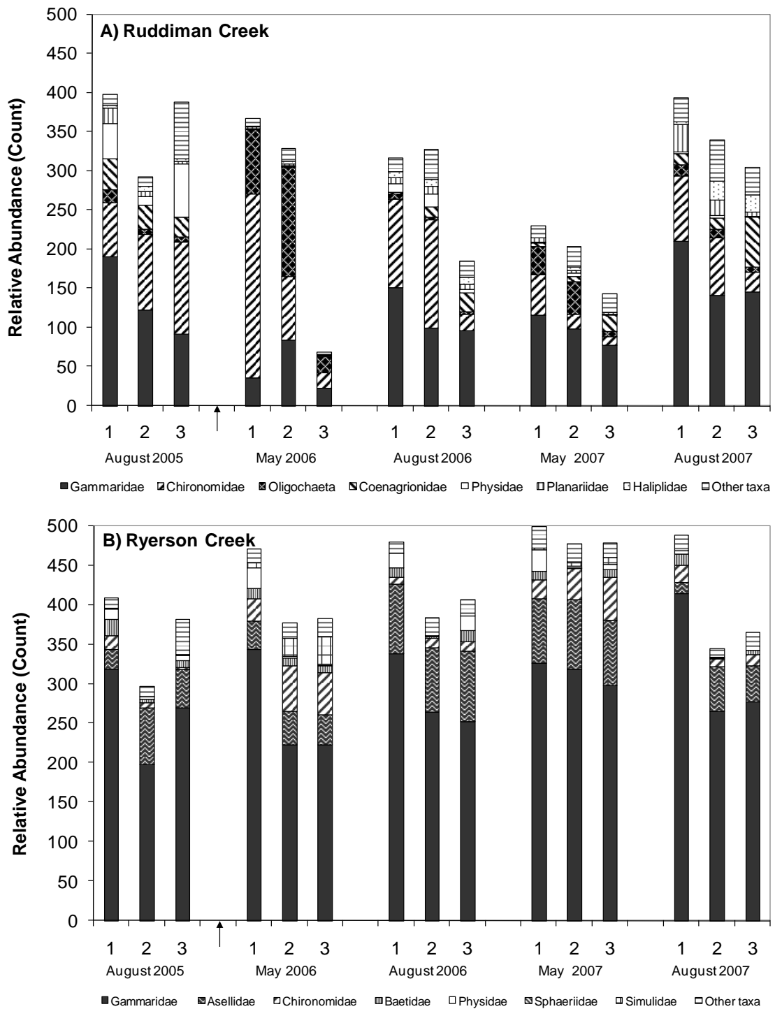
Fig. 7. Mean relative abundances of macroinvertebrate taxa collected from Ruddiman and Ryerson Creeks. Arrow (↑) indicates the division between pre and post-remediation.
