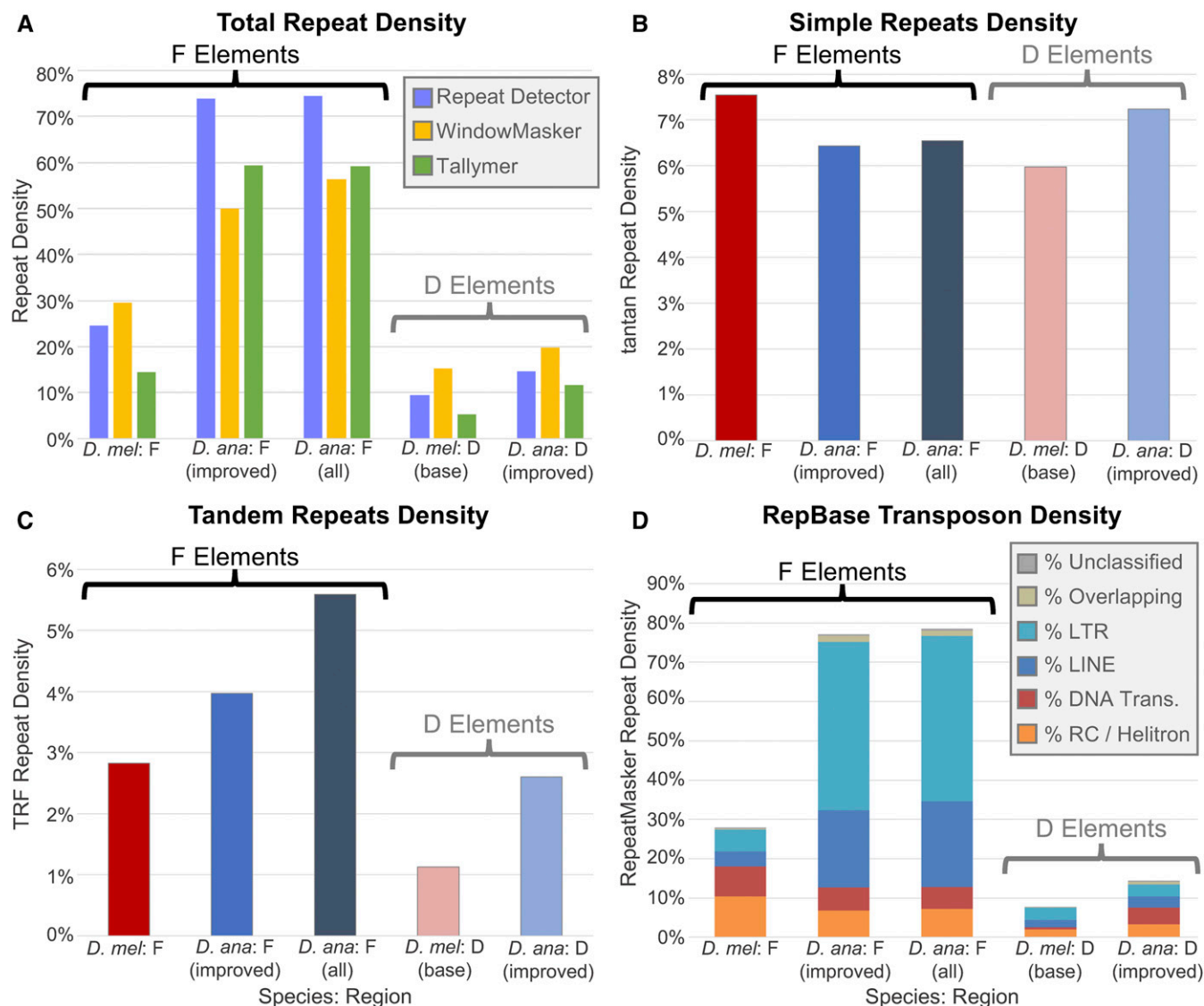
Figure 2 Expansion of the D. ananassae F element can primarily be attributed to the high density of LTR and LINE retrotransposons. (A) Total repeat density estimates from de novo repeat finders (Red, WindowMasker, and Tallymer) show that the D. ananassae F element has higher repeat density than the D. melanogaster F element (56.4–74.5% vs. 14.4–29.5%). Both F elements show higher repeat density than the euchromatic reference regions from the base of the D elements in D. ananassae (11.6–19.8%) and in D. melanogaster (5.4–15.2%). The repeat densities of the improved D. ananassae F-element scaffolds [ D. ana : F (improved)] are similar to the repeat densities for all D. ananassae F-element scaffolds [ D. ana : F (all)]. (B) Results from the tantan analysis show that the five analysis regions from D. melanogaster and D. ananassae have similar simple repeat density (6.0–7.5%). (C) TRF analysis shows that D. ananassae has higher tandem repeats density than D. melanogaster on both the F (5.6 vs. 2.8%) and the D elements (2.6 vs. 1.1%). (D) RepeatMasker analysis using the Drosophila RepBase library shows that the F element has higher transposon density than the D element both in D. melanogaster (28.0 vs. 7.7%) and in D. ananassae (78.6 vs. 14.4%). There is a substantial increase in the density of LTR and LINE retrotransposons on the D. ananassae F element compared to the D. melanogaster F element (42.1 vs. 5.5% and 21.8 vs. 3.8%, respectively). The D. ananassae euchromatic reference region also shows higher transposon density than D. melanogaster , but most of the difference can be attributed to the density of DNA transposons (4.3 vs. 0.6%). The region of overlap between two repeat fragments is classified as “Overlapping” if the two repeats belong to different repeat classes.
