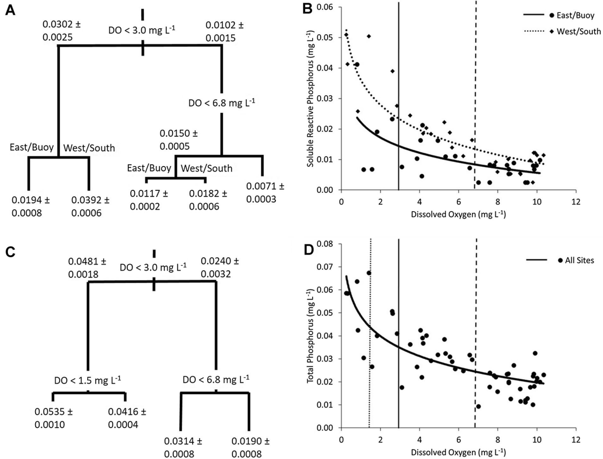
Figure 4. A CART analysis for soluble reactive phosphorus (SRP). Numbers at corners and end of lines represent concentrations mg L -1 ± variance. When a division occurs at DO, less than that DO goes left and more than goes right. When division occurs at site location, similar groups of sites are labeled at corners, B graph of SRP versus DO. Curved lines represent the log regression for East/Buoy ( solid ) and West/South ( dotted ). Vertical lines are for the tree divisions at 3.0 mg L -1 ( solid ) and 6.8 mg L -1 ( dashed ) DO, C CART analysis for total phosphorus (TP). Follows same interpretation as A , D graph of TP versus DO. Solid curved line represents the log regression for all sites combined. Vertical lines represent the tree divisions at 1.5 mg L -1 ( dotted ), 3.0 mg L -1 ( solid ), and 6.8 mg L -1 ( dashed ) DO.
