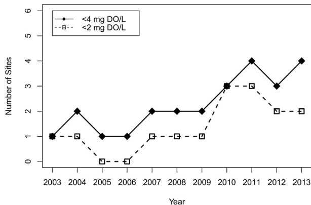
Fig. 7. Number of sites in the month of July (summer) where bottom water was either mildly hypoxic ( < 4 \text{ mg DO l}^{-1} ) or severely hypoxic ( < 2 \text{ mg DO l}^{-1} ) during seasonal monitoring of 6 sites through years 2003–2013 in Muskegon Lake. Note: We did not expect hypoxia to occur at all 6 sites since 2–3 sites in the long-term seasonal survey are too shallow to experience hypolimnion.
