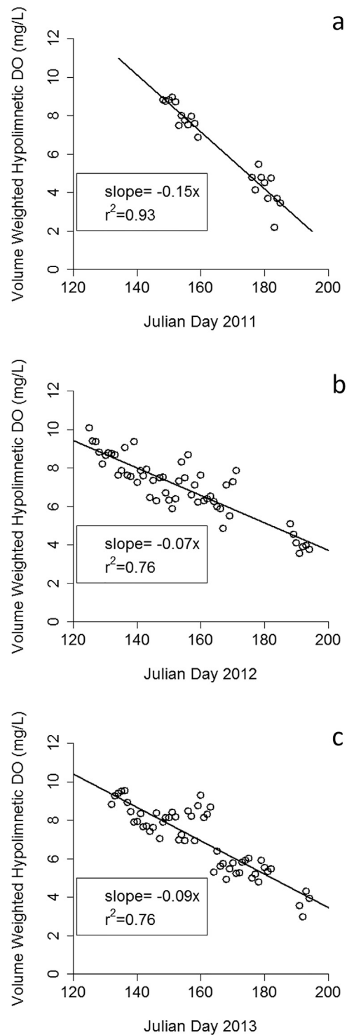
Fig. 4. Volumetric Hypolimnetic Oxygen Depletion estimates (VHOD obs ) during 2011 (a), 2012 (b) and 2013 (c), based on measured change in volume-weighted DO in the hypolimnion. Rate units are in \text{mg O}_2 \text{ l}^{-1} \text{ d}^{-1} as represented by the regression slope of DO over Julian days.
