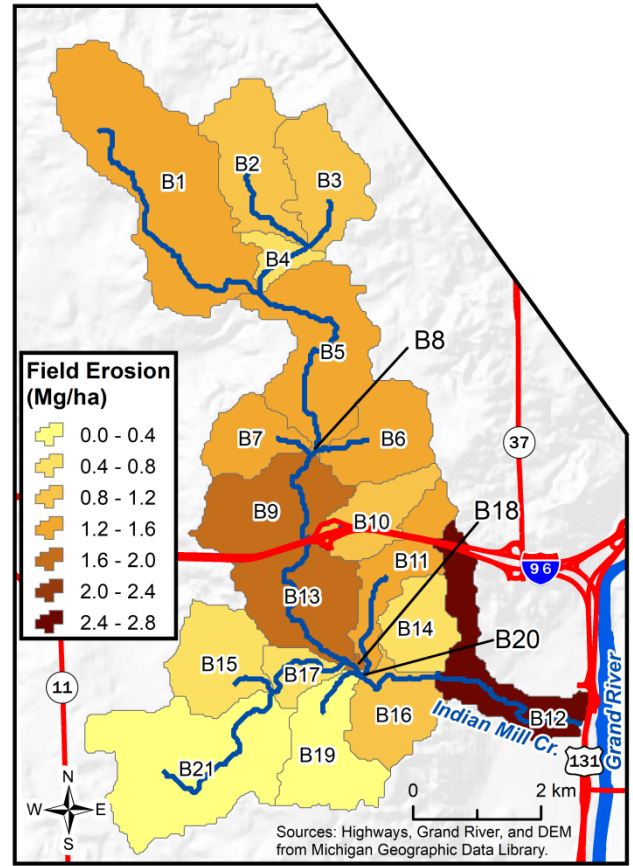
Figure 3.6. Annual field erosion results from the GWLF-E model for subbasins in the Indian Mill Creek watershed 1997-2015.
