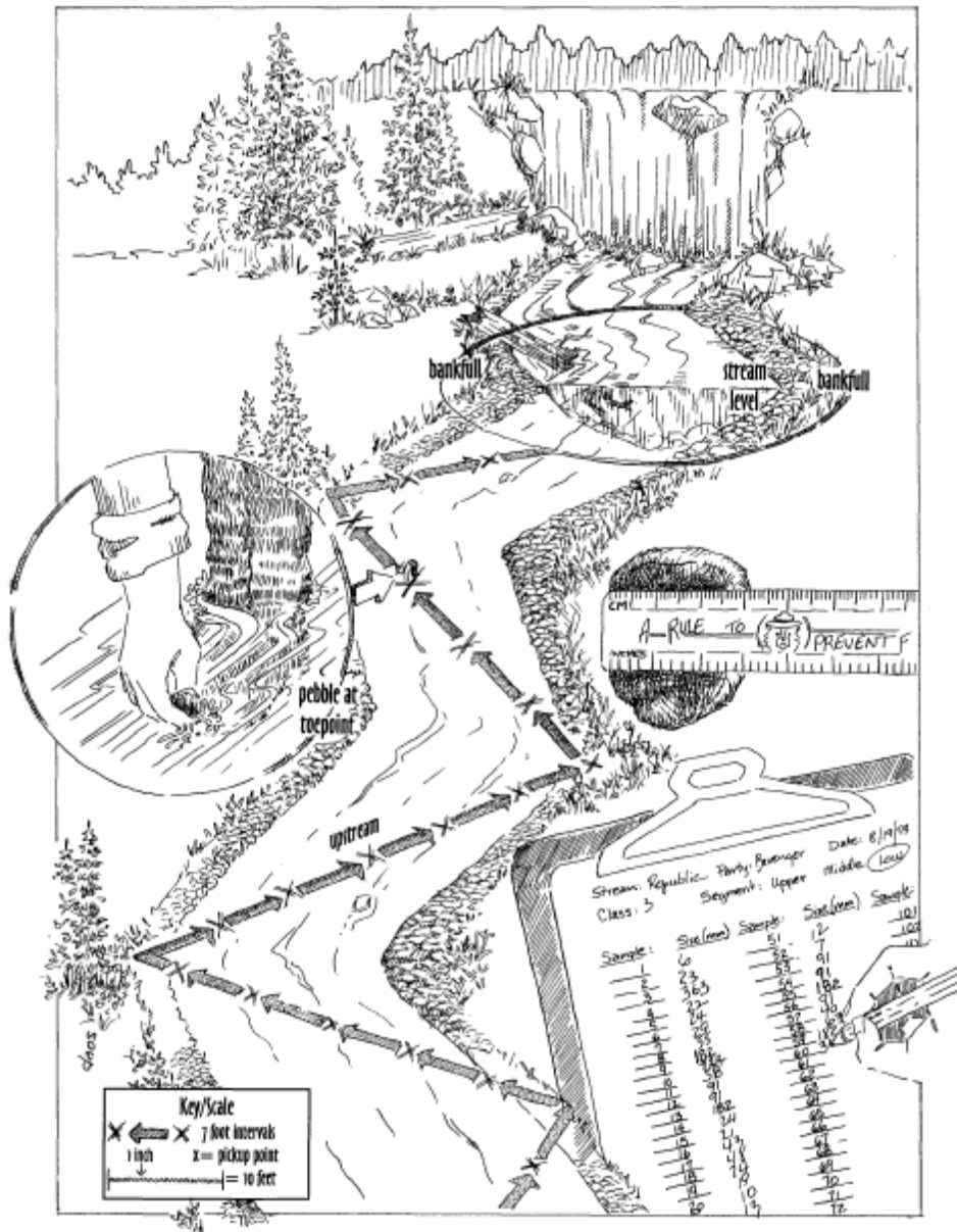
Figure 6.2. Zig-zag method for pebble counts (Beverger and King 1995).
