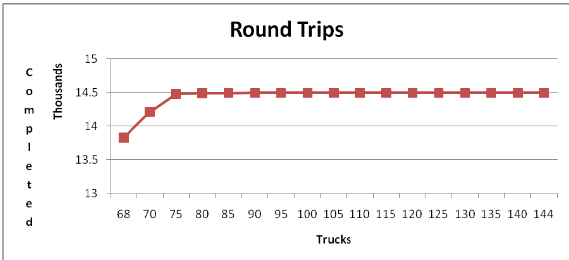
Figure 14-3: Round Trips versus Number of Trucks
